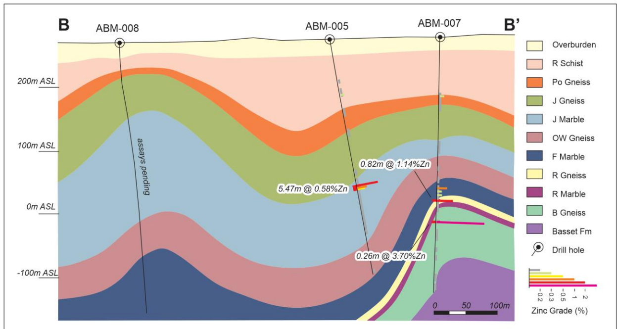
Figure 3: Cross section B-B' with significant zinc intercepts, Mountain Zinc-Copper Project, Virginia. View looking northeast.
