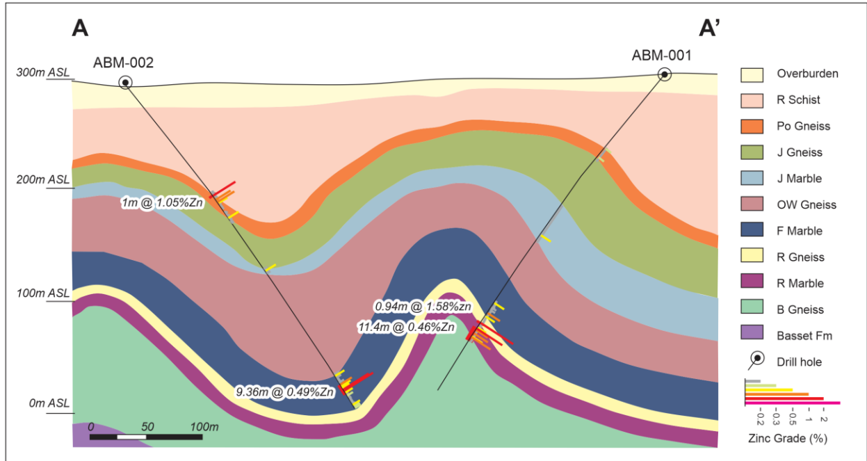
Figure 2: Cross section A-A' with significant zinc intercepts, Mountain Zinc-Copper Project, Virginia. View looking northeast.
