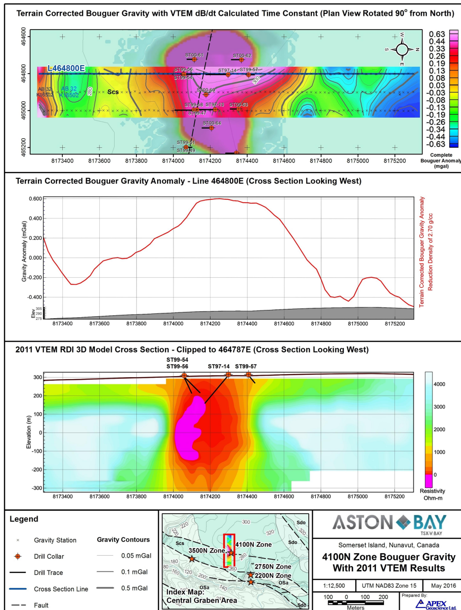
Figure 9.5 4100N Zone Bouguer Gravity and 2011 VTEM Results
